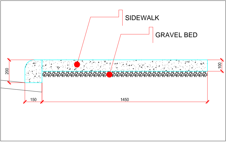
2 TYPICAL SECTION OF SIDEWALK A-02 SCALE 1:200
